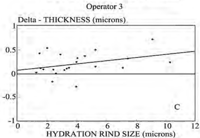
Figure 3. Delta-T vs. rind thickness. Solid line shows trend in readings.
